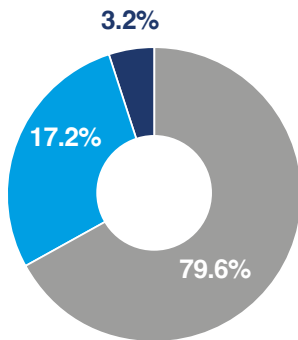
Saudi Arabia
